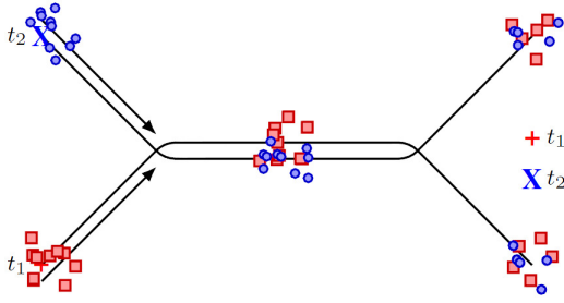
Figure 2: Particle representation of the multi-target distribution in a situation where mixed labelling occurs ([5])
