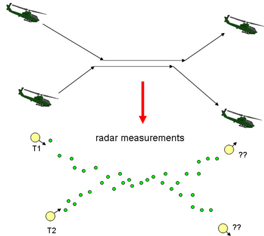
Figure 1: Situation where assignment of labels to tracks is ambiguous
